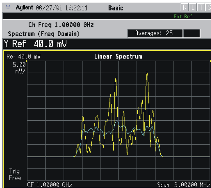
Figure 3-2 Spectrum Measurement - Linear Spectrum View (for E4406A)
