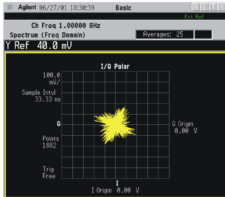
Figure 3-4 Spectrum Measurement - I/Q Polar View (for E4406A)
