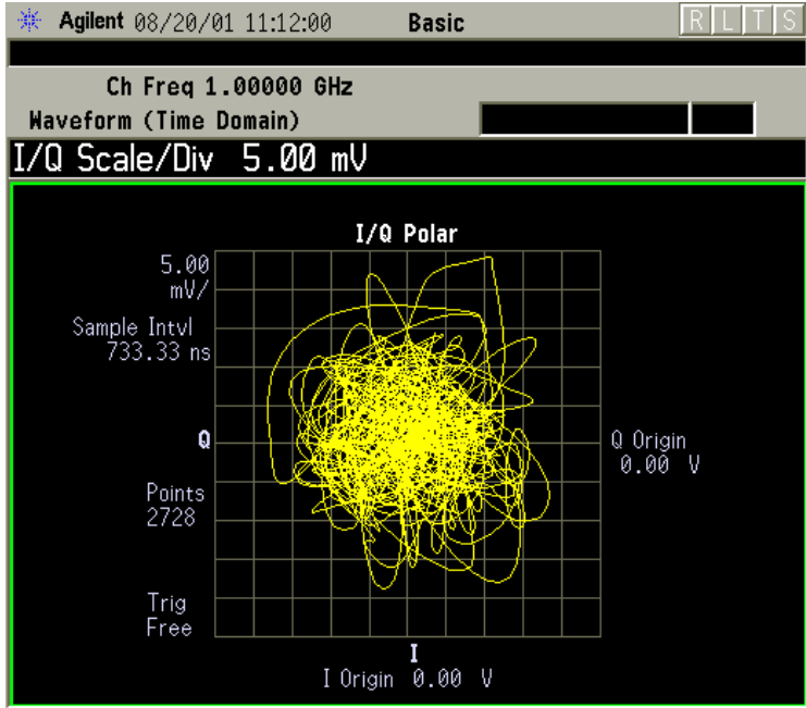
Figure 3-8 Waveform Measurement - I/Q Polar View
