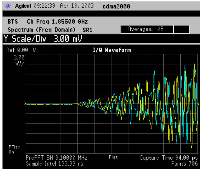
Figure 2-3 Spectrum Measurement - I/Q Waveform (Time Domain) Result
