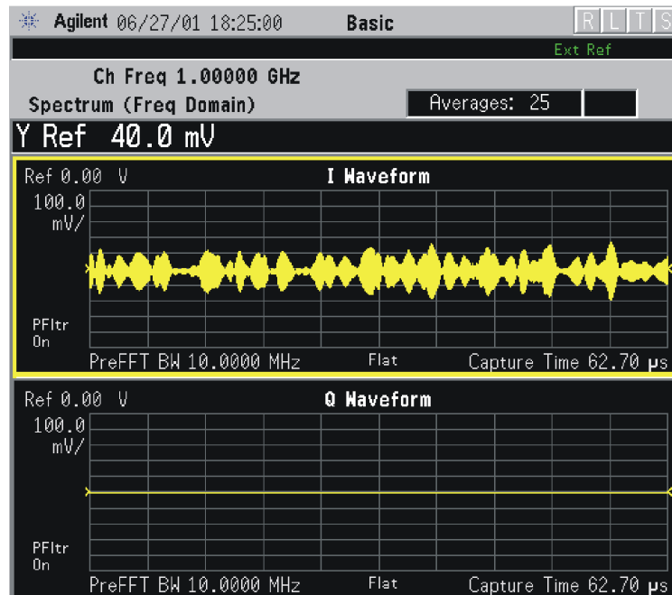
Figure 3-3 Spectrum Measurement - I and Q Waveform View (for E4406A)
