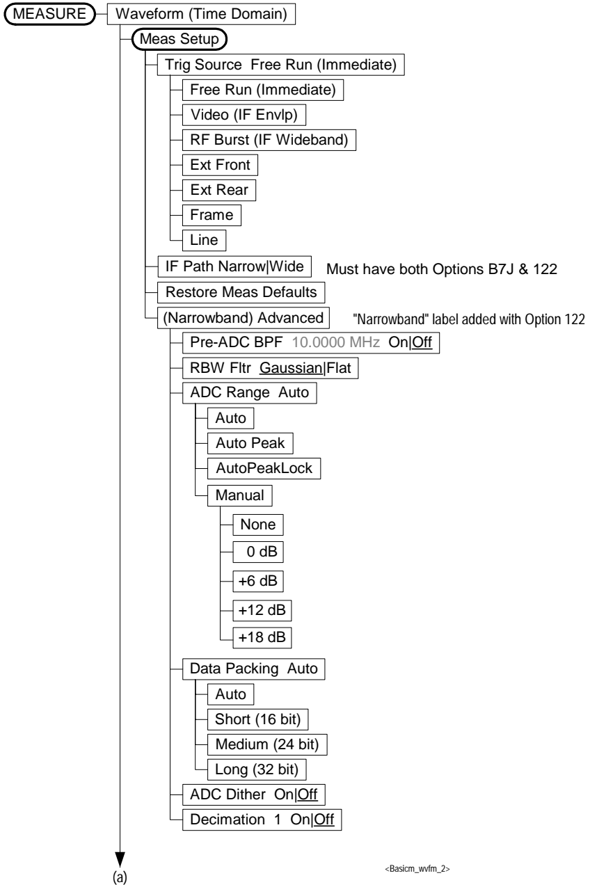
Figure 6-8 Waveform (Time Domain) Measurement Key Flow (2 of 3)
