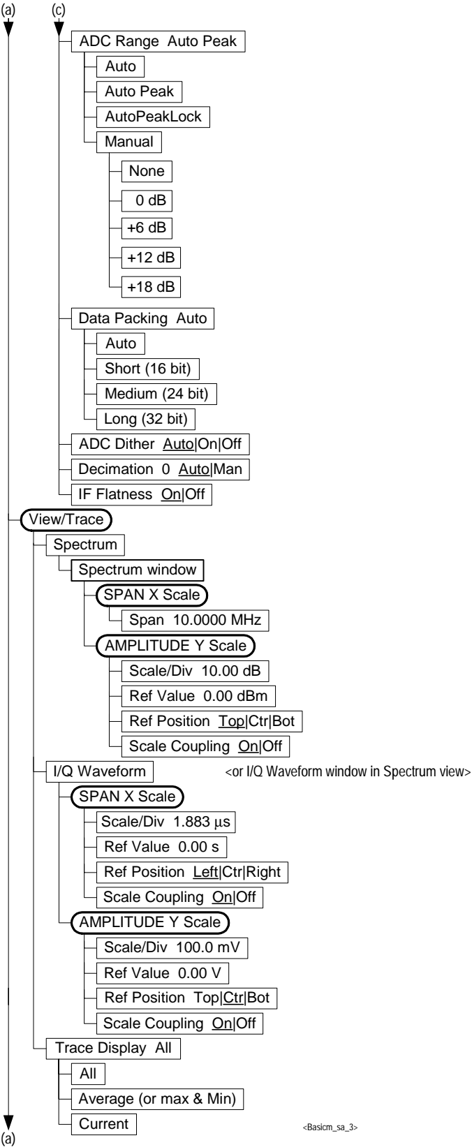
Figure 6-5 Spectrum (Freq Domain) Measurement Key Flow (3 of 4)
