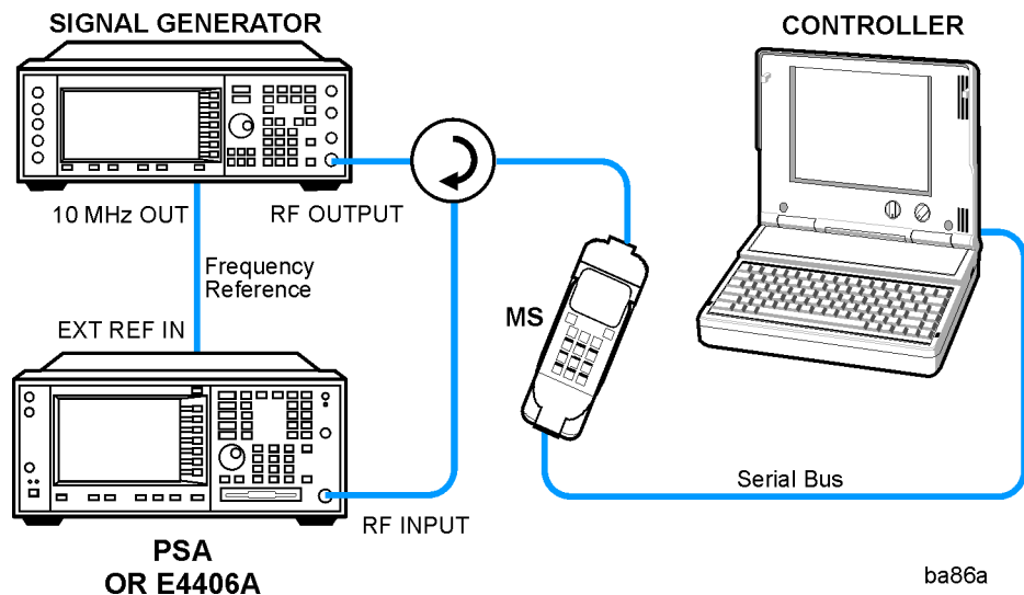
Figure 2-4 Waveform Measurement System
