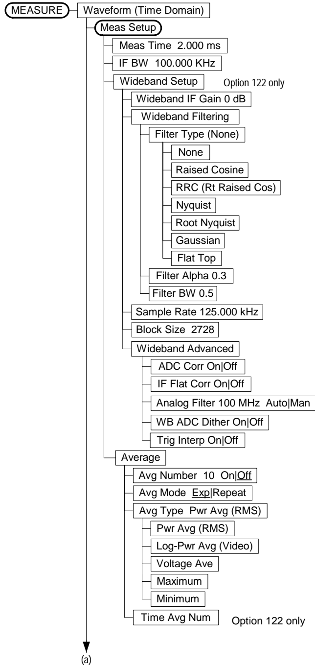
Figure 6-7 Waveform (Time Domain) Measurement Key Flow (1 of 3)
