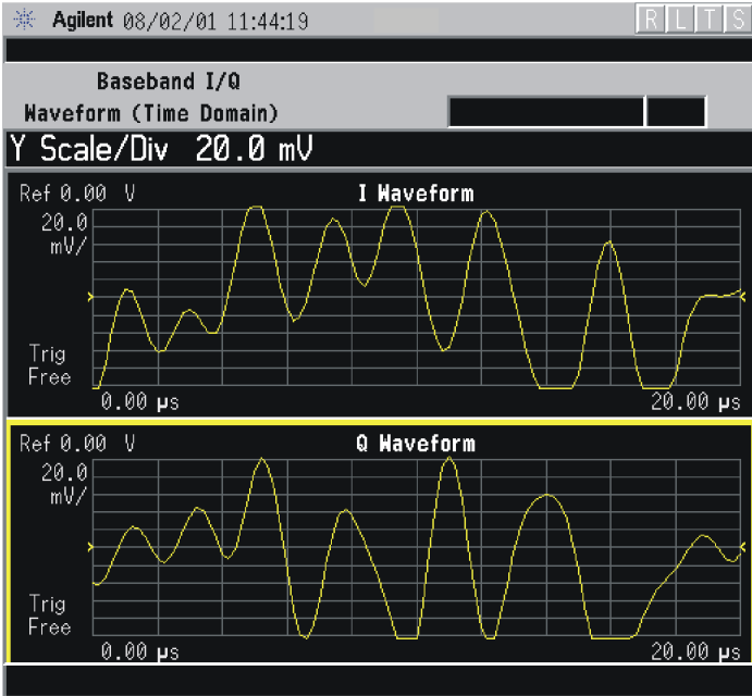
Figure 3-7 Waveform Measurement - I and Q Waveform View
