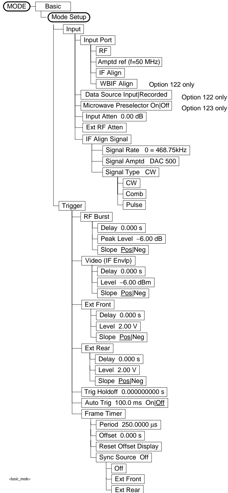
Figure 6-1 Mode Setup Key Flow
