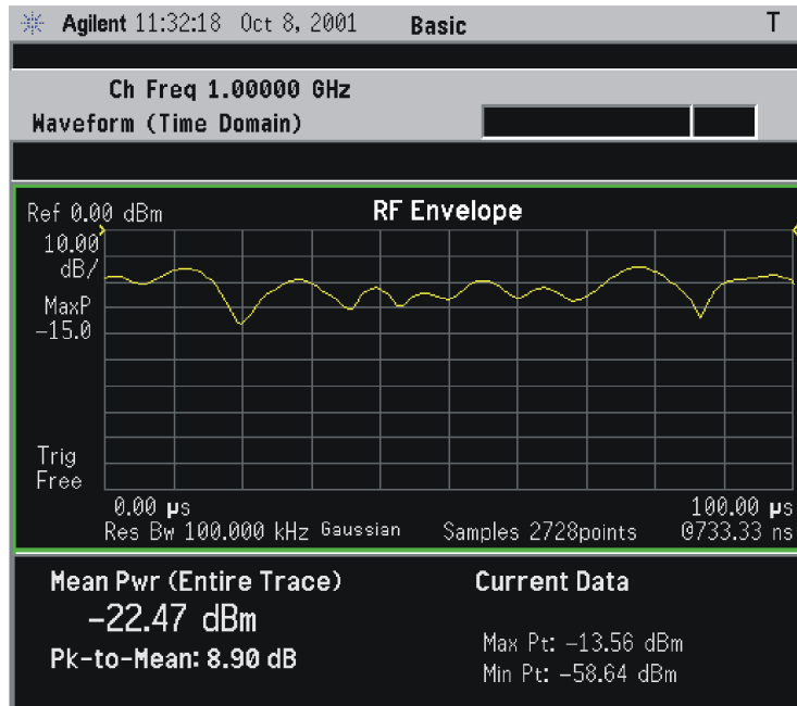
Figure 2-5 Waveform Measurement - RF Envelope (Default View)
